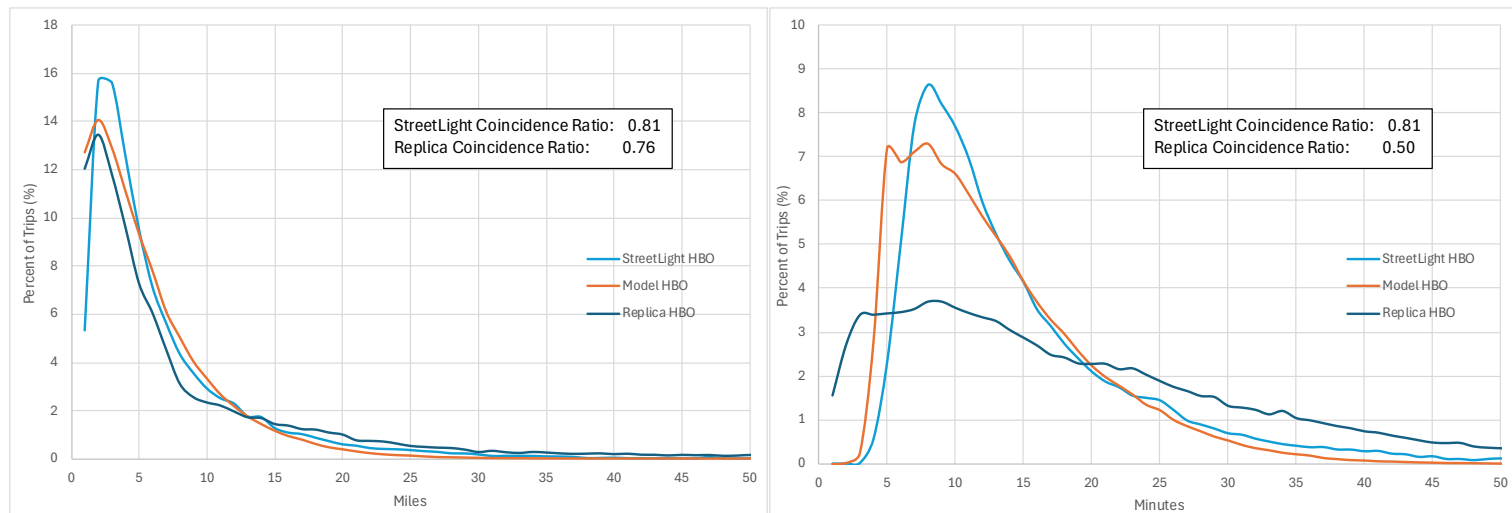
Figure 9 - Home-Based Other Trip Length Distribution Curves (Miles and Minutes)
