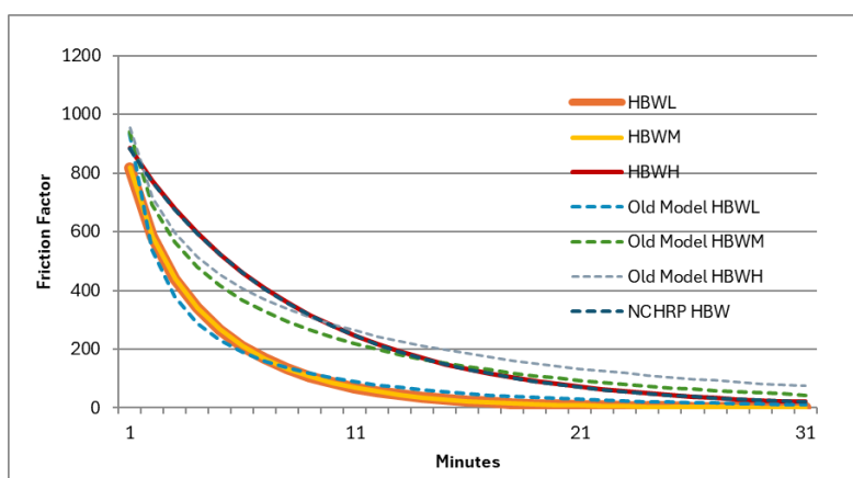
Figure 11 - HBW Friction Factor Curves (All Income Levels)
