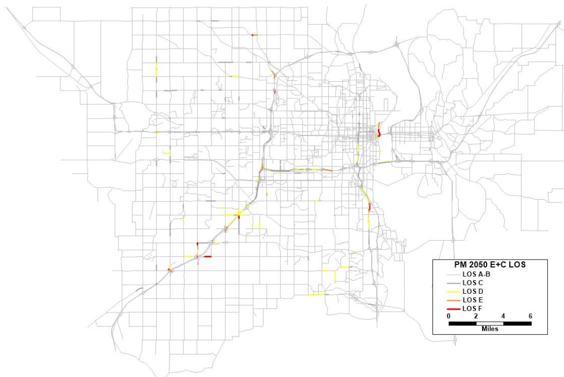
Figure 24 - 2050 Committed PM Level-of-Service
