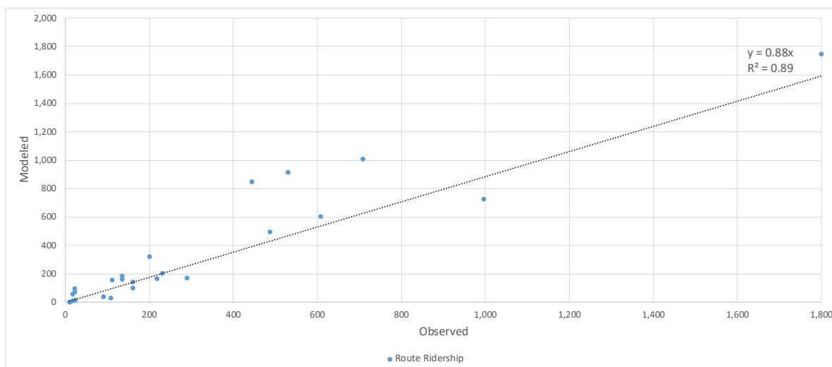
Figure 16 - Observed Versus Modeled Ridership by Route
