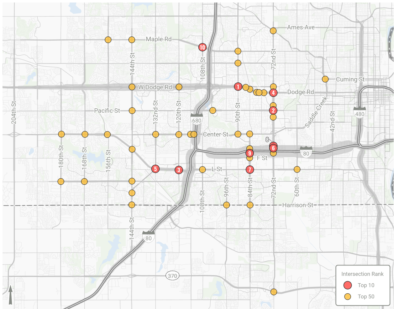
Figure 1: Top 50 Intersections
