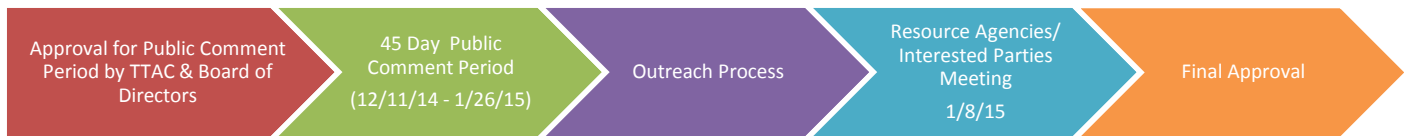
Figure 1.2: Development Methodology
